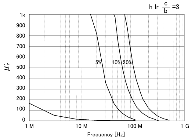
Figure 29. Permeability ( \mu' ) vs. frequency (at F = 3 , typical)
