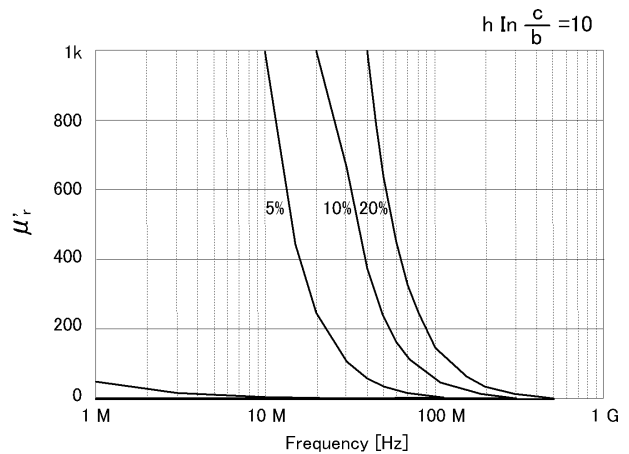
Figure 30. Permeability ( \mu' ) vs. frequency (at F = 10 , typical)
