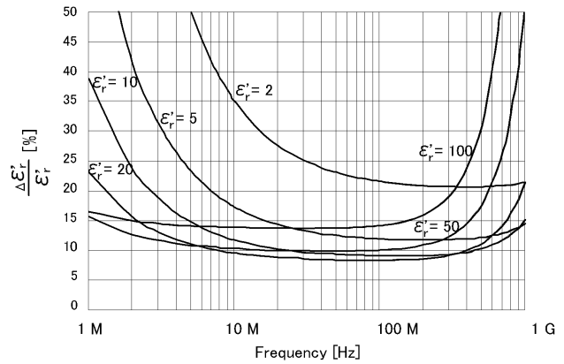
Figure 15. Permittivity accuracy \frac{(\Delta \epsilon'_r)}{\epsilon'_r} vs. frequency (at t = 3 mm, typical)
