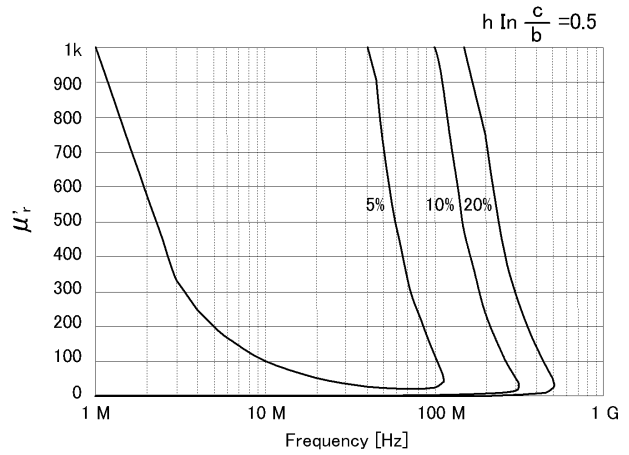
Figure 28. Permeability ( \mu' ) vs. frequency (at F = 0.5 , typical)
